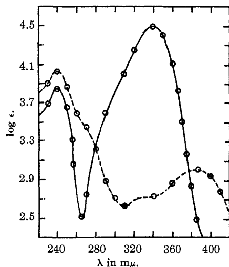
Fig. 2.— — p -Dimethylaminobenzaldehyde; ---, 2-dimethylamino-5-methylbenzaldehyde.
