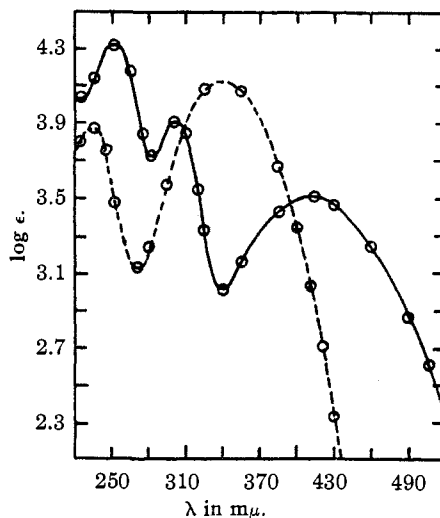
Fig. 4.— — Orange compound, sodium salt; ---, ethyl aceto-pyruvate-anil.
